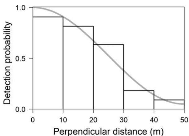
FIG. 2 Distribution of perpendicular distances of observations of M. marcai on transects in the Marmelos–Ariupaná interfluvium (Fig. 1). The trend line indicates the best detection function fitted to the distance classes.
